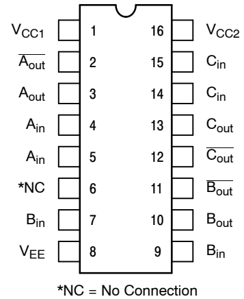
Figure 2. Pin Assignment
