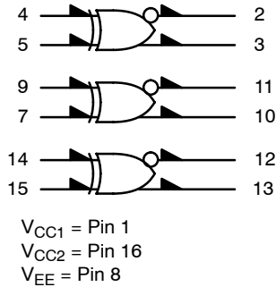
Figure 1. Logic Diagram
